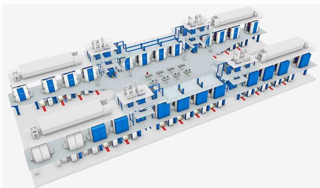
West Ferry Printers' CT-Commander configuration, split-up into four presslines.
